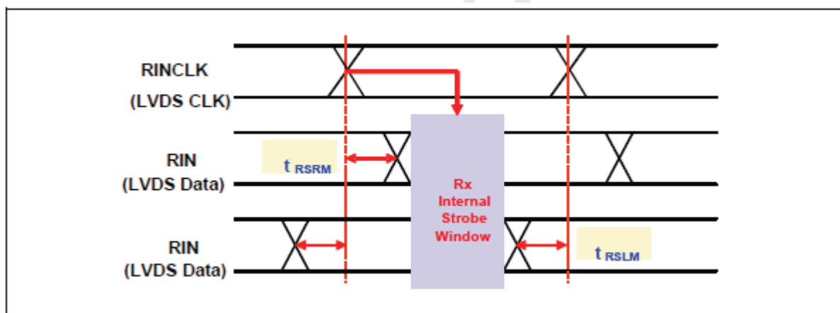
&lt; LVDS Receiver Skew (Strobe) Margin &gt;
