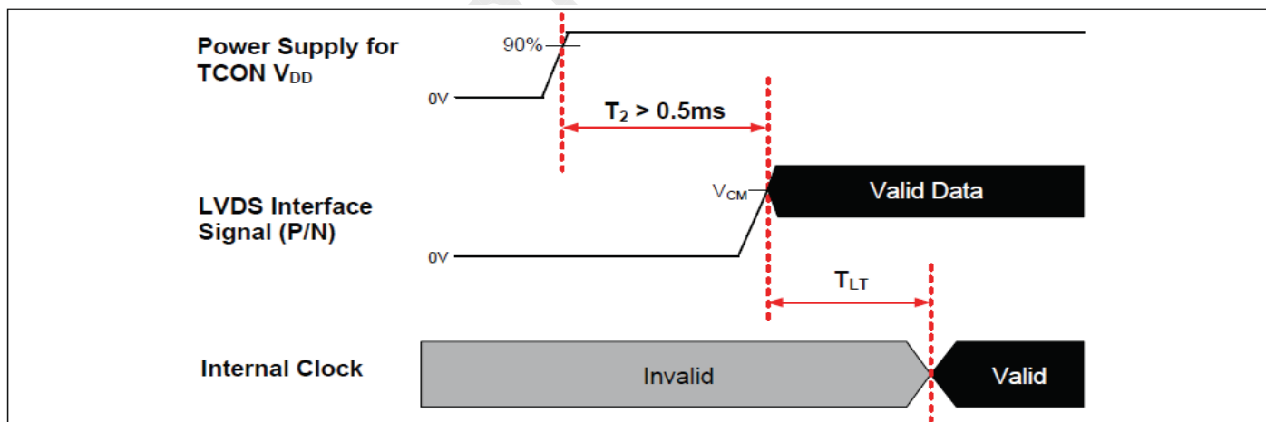
< Timing Diagram of LVDS Operation >
